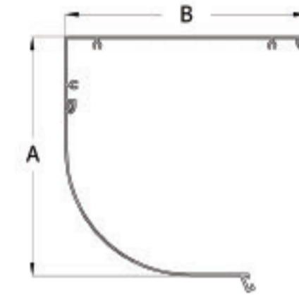
EXTRUDED ALUMINIUM HALF ROUND FRONT BOX (145mm, 170mm)
