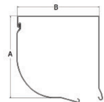
ALUMINIUM HALF ROUND FRONT BOX (137mm)
