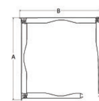
THERMO INSULATED ALUMINIUM BOX (147mm, 172mm, 195mm)
